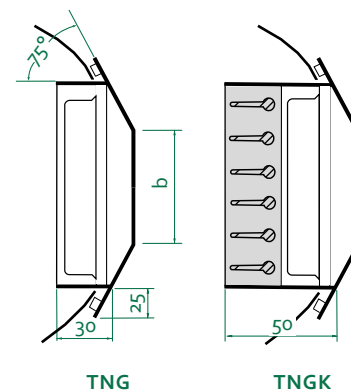
Dimensions of duct grilles
