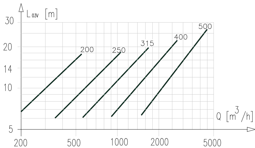
Selection diagram according to isothermal vertical jet throw
